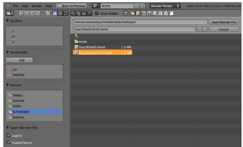
Abb. 3-3 File Window
