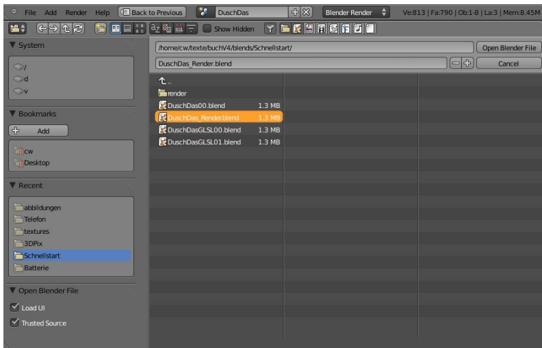
Abb. 3–9 File Window
