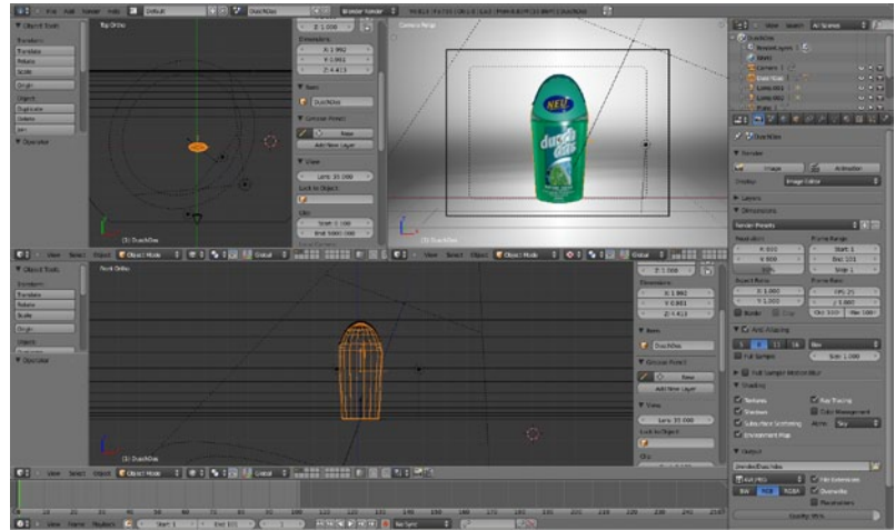
Abb. 3–10 Render-Schnellstart
